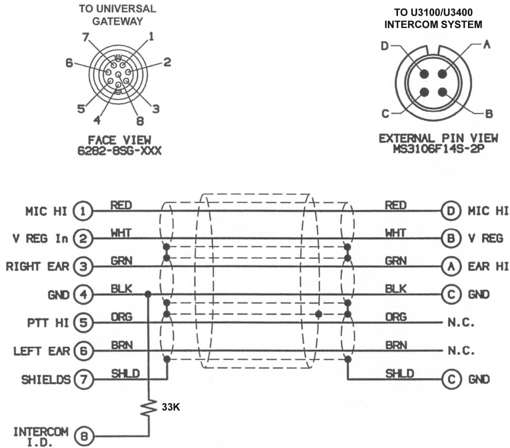
Fig. 2 Cable Schematic, Universal Gateway to 3100/3400
