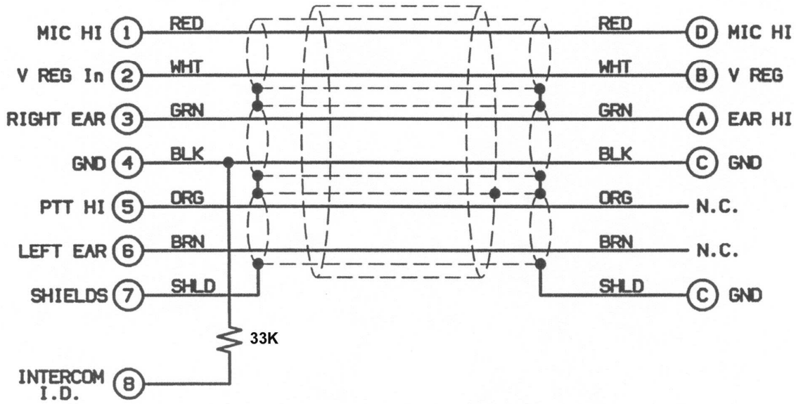
Fig. 3 Cable Schematic, 3800 Gateway to U9925-GEM
